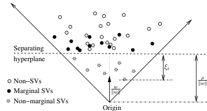
Figure 1. This figure illustrates the geometric interpretation of optimal hyperplane for one class SVMs.
